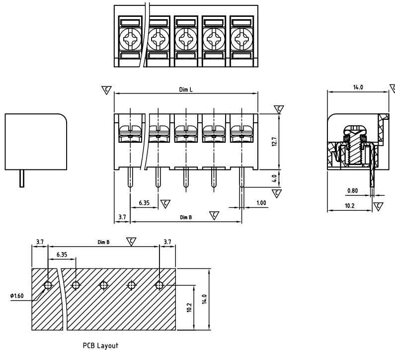
PCB Layout
